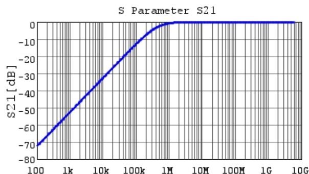
GRM155R71H392KA01 S21 DC0V, 25degC
