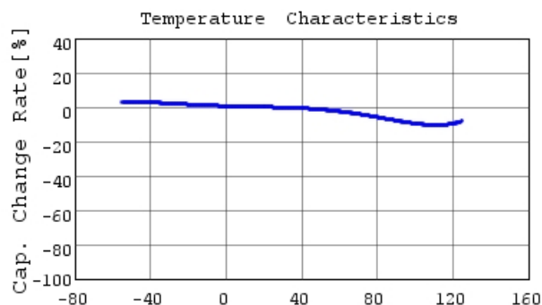
GRM155R71H392KA01 C-Temp. capchange, DC0.0V,
