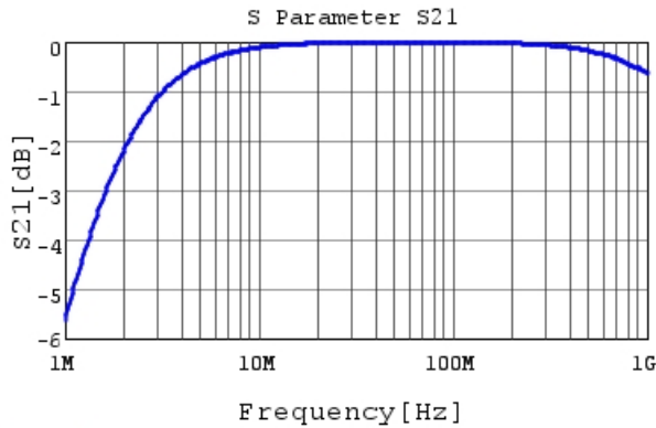
RHE5G1H102J0K1H03B S21 DCOV, 25degC
