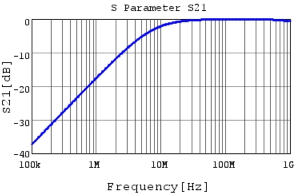
RHEL81H221K0M1H03A S21 DCOV, 25degC
