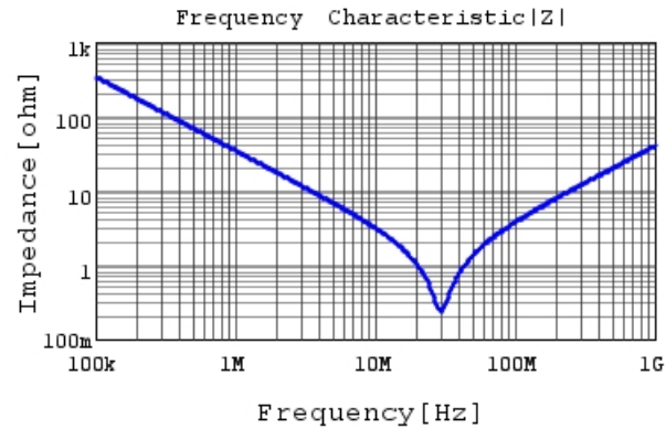
RHEL81H472K0M1H03A |Z| DCOV,25degC
