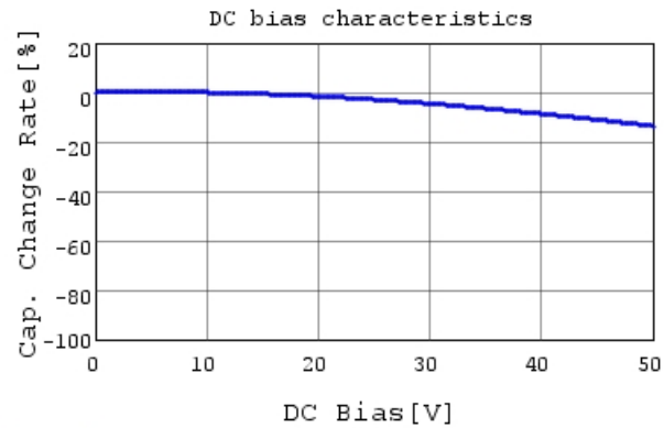
RHEL81H472K0M1H03A C-DC bias capchange, 25.0
