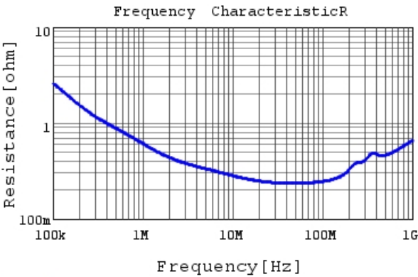
RHEL81H472K0M1H03A R DCOV,25degC
