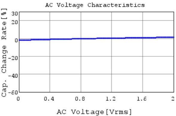
RHEL81H472K0M1H03A C-AC Voltage capchange, I
