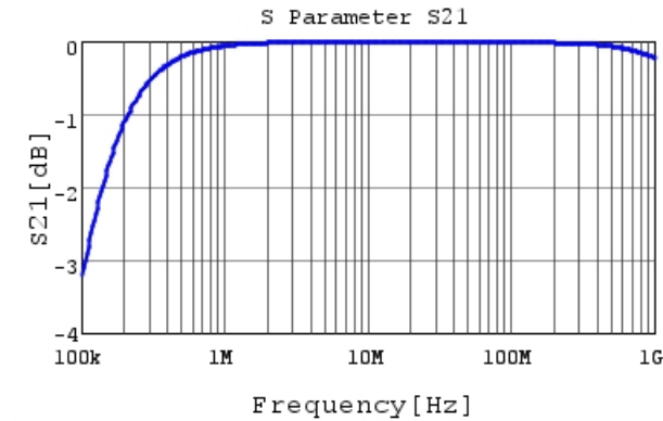
RHEL82A153K0A2H03B S21 DCOV, 25degC
