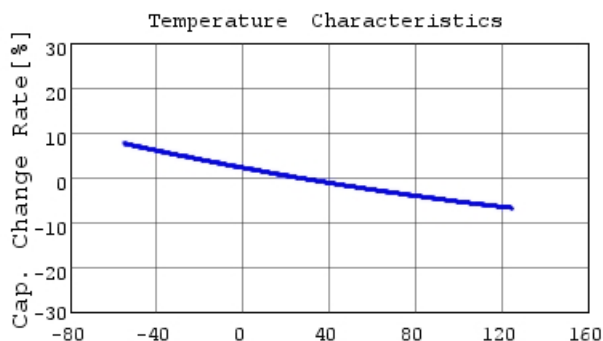
Temperature [degC] GCM1887U2A392JA16 C-Temp. capchange, DCOV, 1
