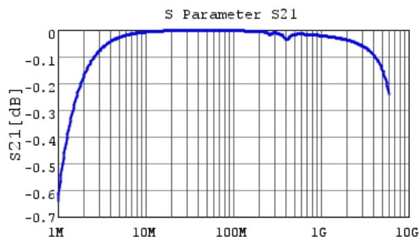
Frequency [Hz] GCM1887U2A392JA16 S21 DCOV, 25degC
