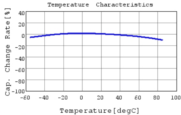
GRM011R60J104ME01 C-Temp. capchange, DC0.0V,
