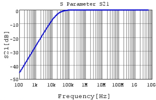
GRM011R60J104ME01 S21 DC0V,25degC
