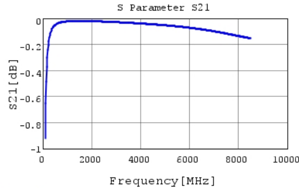
GRM0225C1H330JA02 S21 DCOV, 25degC
