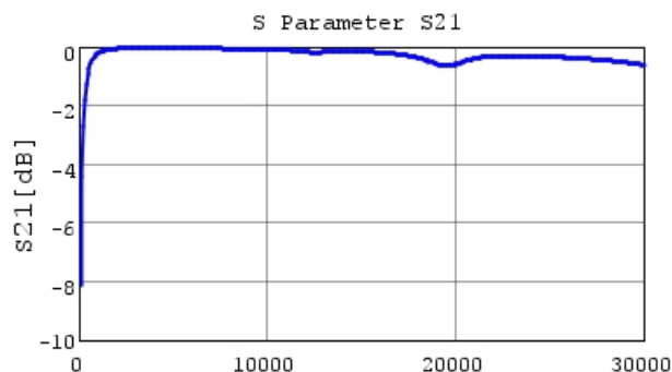
GRM0225C1H6R8DA03 S21 DCOV, 25degC
