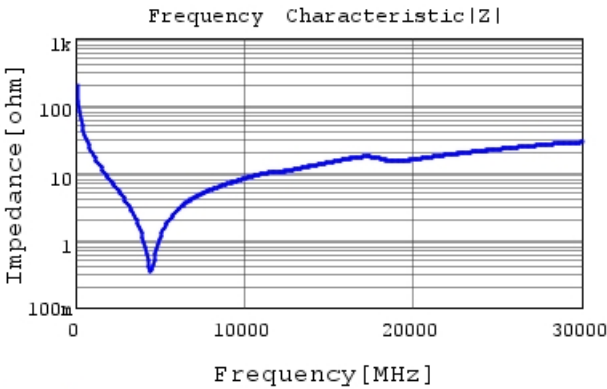
GRM0225C1H7R8BA03 |Z| DCOV,25degC
