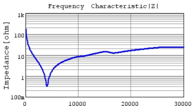
GRM0225C1H9R5DA03 |Z| DCOV,25degC
