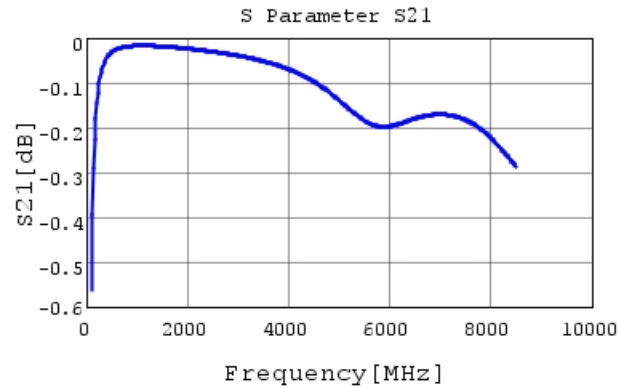
GRM0332C2A430JA01 S21 DCOV, 20degC
