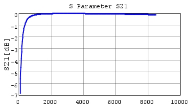
GRM0332C2A8R1CA01 S21 DCOV, 20degC
