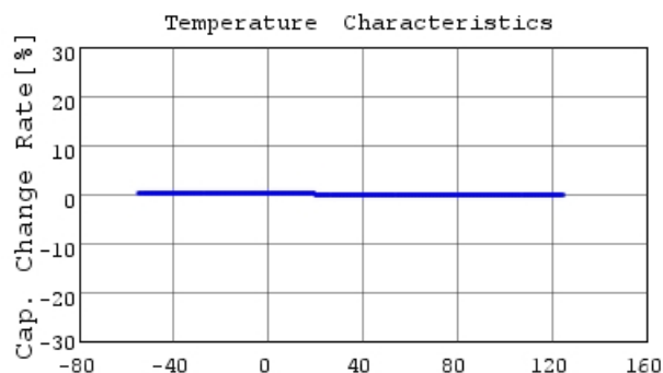
GRM0332C2A8R1CA01 C-Temp. capchange, DCOV, 1
