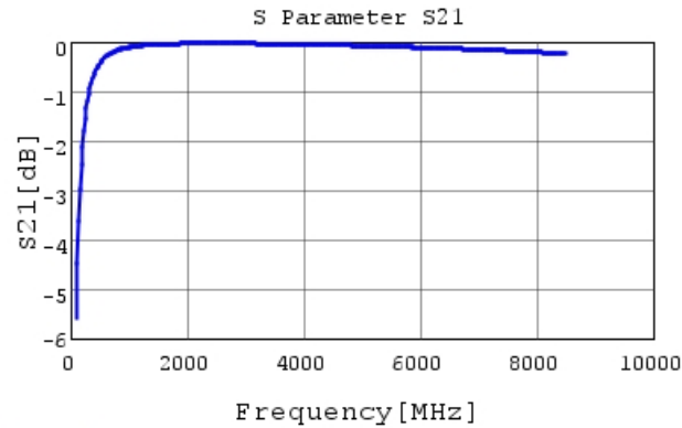
GRM0332C2A9R8DA01 S21 DCOV, 20degC
