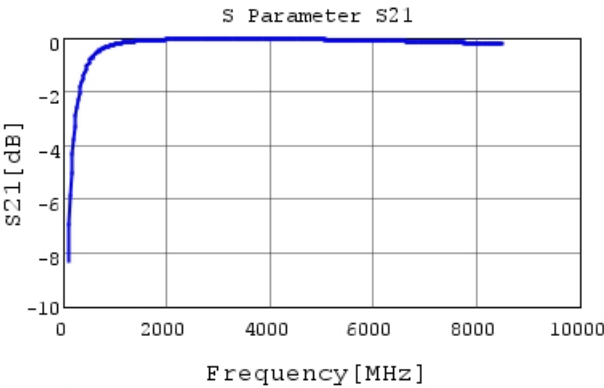
GRM0335C1H6R6WA01 S21 DCOV, 25degC
