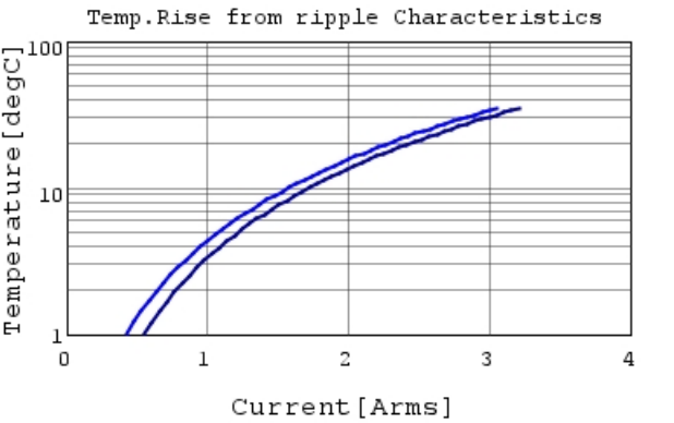
GRM033R61A225KE47 Temp.rise — 500kHz —
