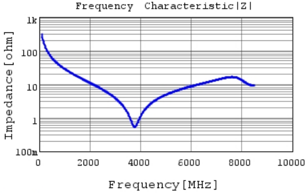
GRM1552C2A5R2DA01 |Z| DCOV, 20degC
