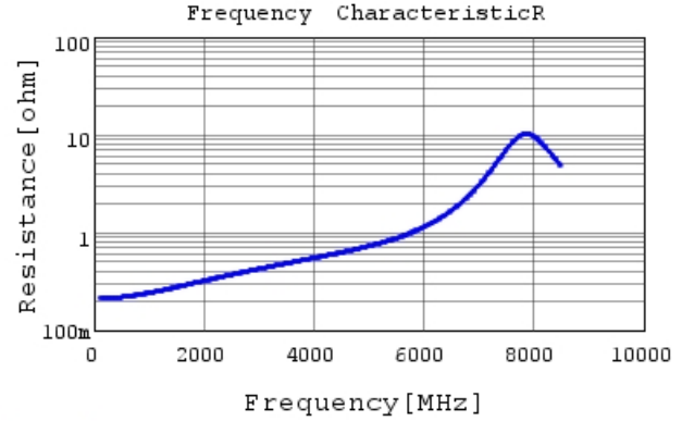
GRM1552C2A5R2DA01 R DCOV, 20degC
