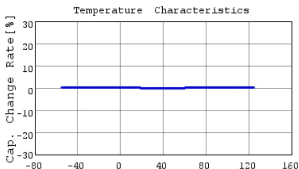
GRM1552C2A6R4DA01 C-Temp. capchange, DCOV, 1
