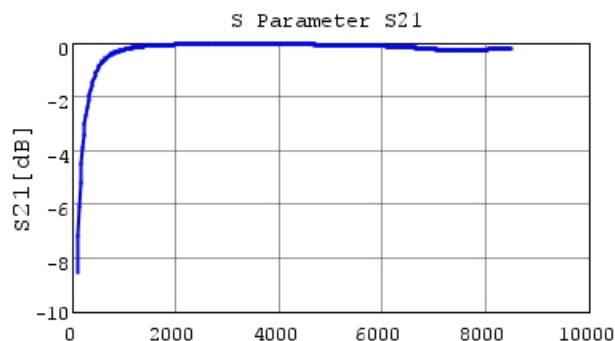
GRM1552C2A6R4DA01 S21 DCOV, 20degC
