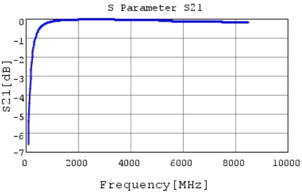
GRM1555C2A8R4BA01 S21 DC0V, 25degC
