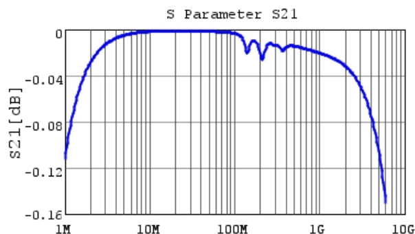
GRM1885C1H103JA01 S21 DCOV, 25degC
