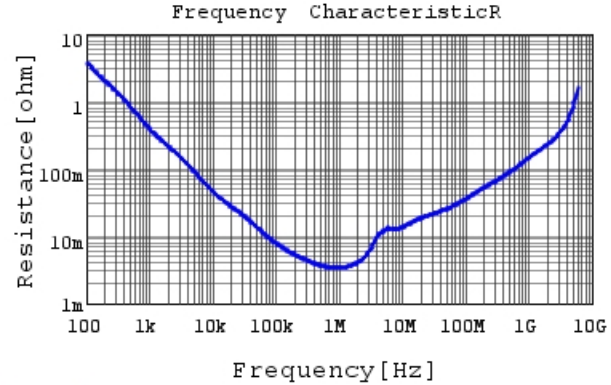
GRM188R61C106MA73 R DCOV,25degC
