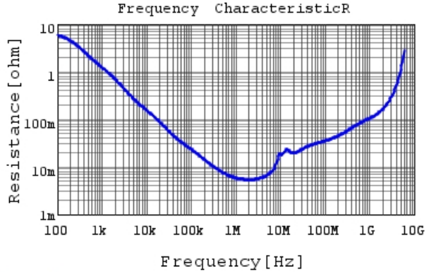
GRM188Z71C225KE43 R DCOV, 25degC
