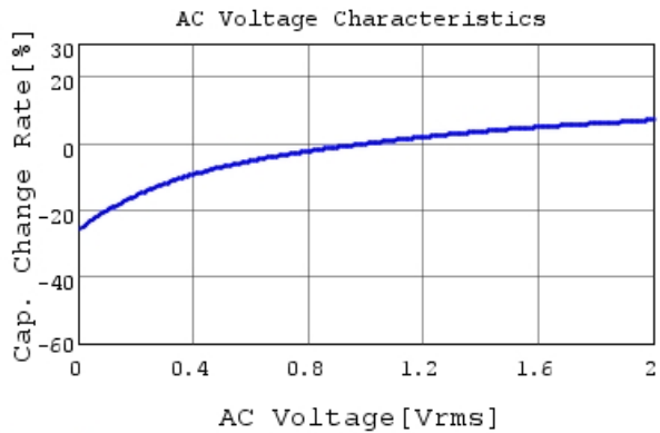
GRM188Z71C225KE43 C-AC Voltage capchange, D
