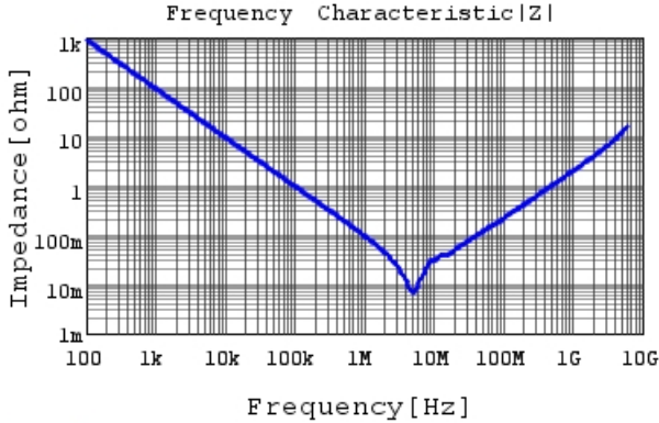
GRM188Z71C225KE43 |Z| DCOV, 25degC
