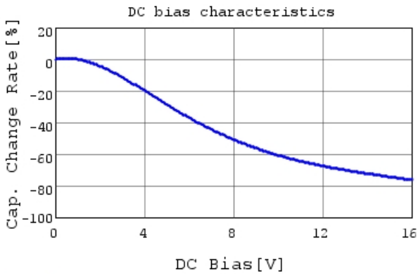
GRM188Z71C225KE43 C-DC bias capchange, 25.0C
