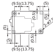
View B
