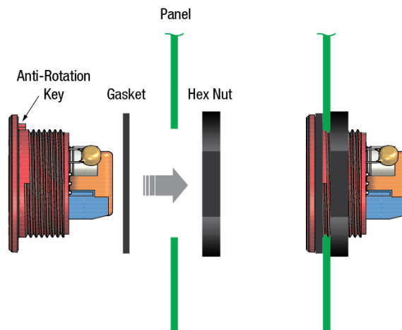
Figure 1. Panel Installation
