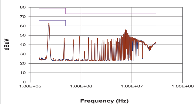
MTC1S2412MC
