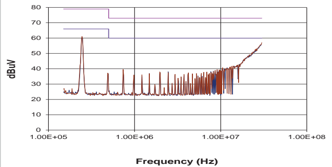
MTC1S2403MC
