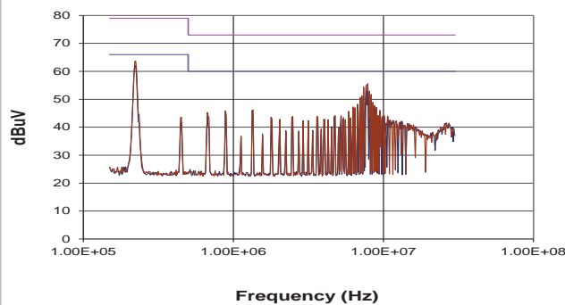
MTC1S2405MC
