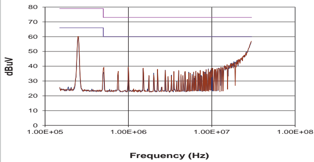
MTC1S1212MC
