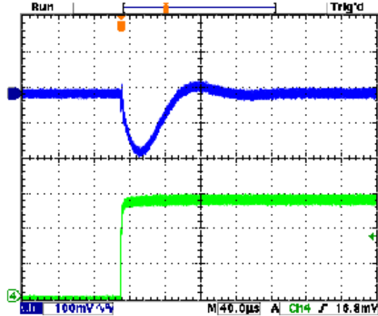
Step Load Transient Response (Vin=12V, Vout=3.3V, Load=10x10µF X5R 0805 ceramic, plus 1x470µF, 7mΩ POSCAP, total 570µF, Iout=0A to 1.5A) Top trace=Vout, Bottom trace=Iout
