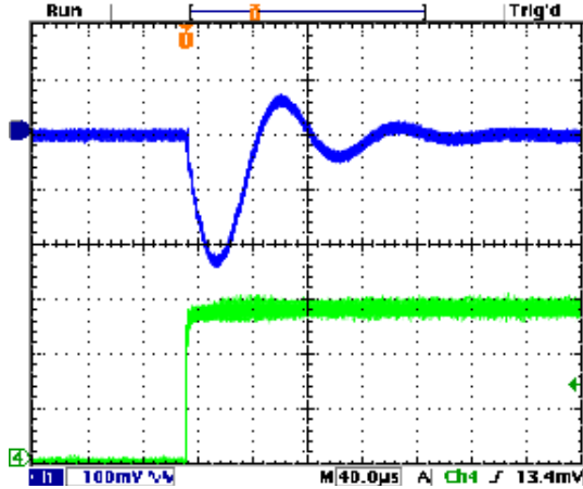
Step Load Transient Response (Vin=4.5V, Vout=1.8V, Cload=10x10µF X5R 0805 ceramic, plus 1x470µF, 7mΩ POSCAP, total 570µF, Iout=0A to 1.5A) Top trace=Vout, Bottom trace=Iout
