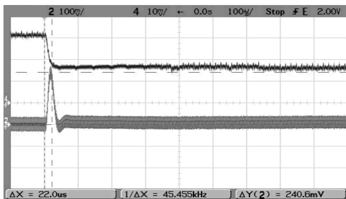
Step Load Transient Response (Vin=12V, Vout=6V, Load=0, Iout=6A to 3A) Trace 2=Vout, 100 mV/div. Trace 4=Iout, 2A/div.
