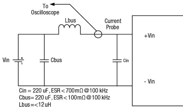
Figure 5. Measuring Input Ripple Current
