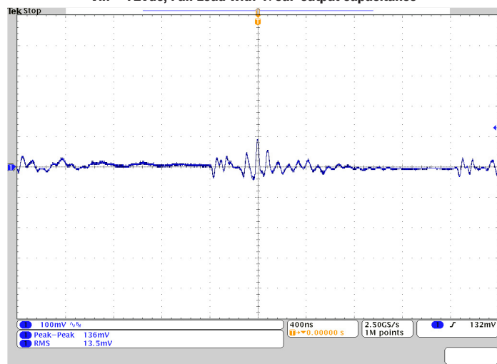
Output Ripple@20MHz BW, Vin = 72Vdc, Full Load with 470uF output capacitance
