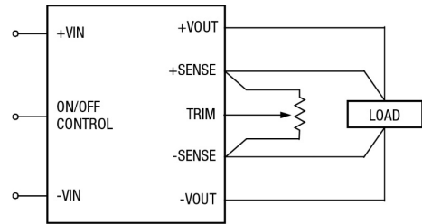
Figure 8. Trim Connections Using a Trimpot
