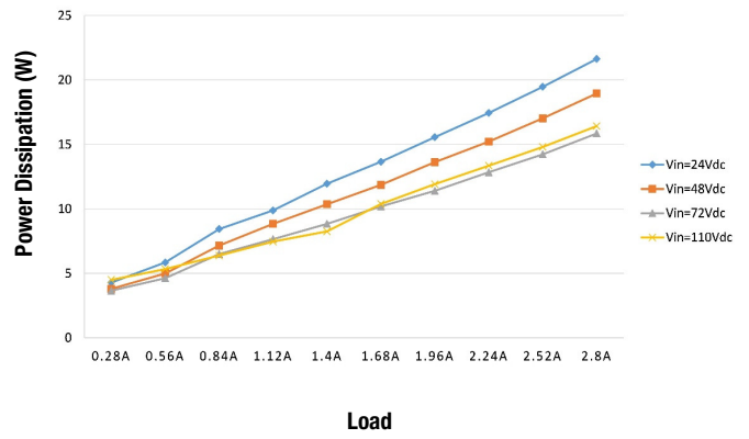
IRQ-54/2.8-W80 Power Dissipation vs Load
