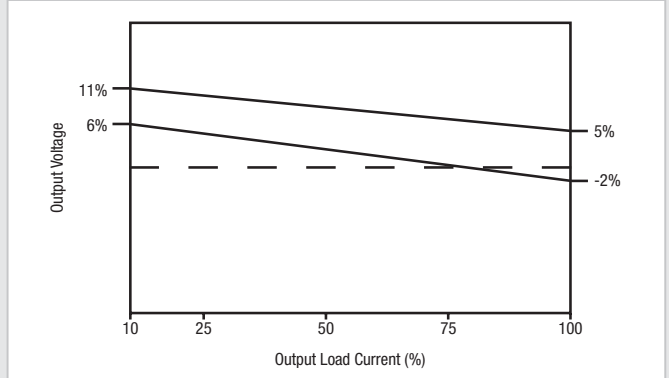
MGJ2D051509MPC
