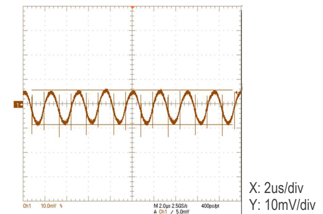
Figure 20. Output Ripple and Noise
