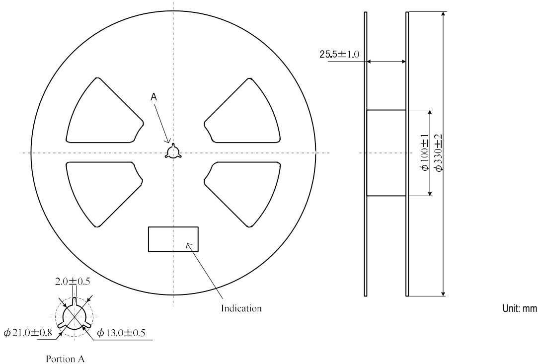
Figure 40. Reel Dimension
