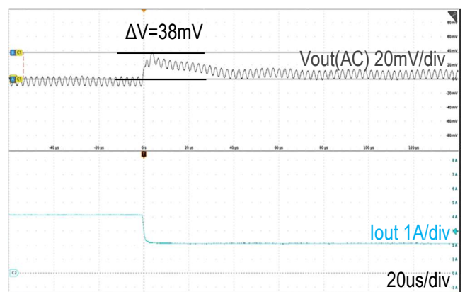
Figure 22. Step Load Transient Response
