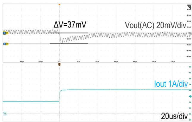
Figure 21. Step Load Transient Response
