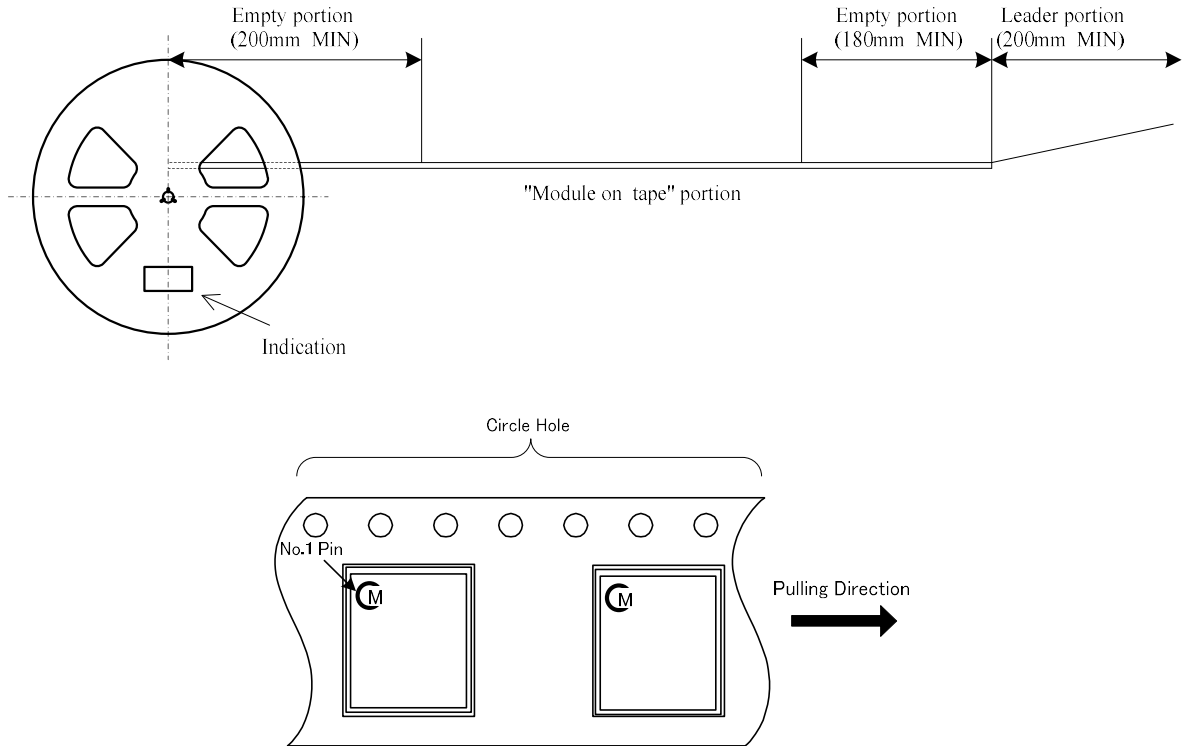
Figure 41. Tape Specifications
