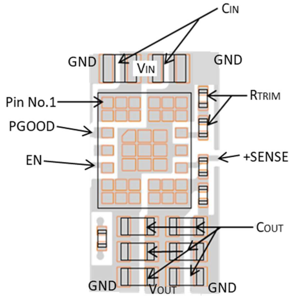
Figure 35. Example of Pattern Layout (Top View)
