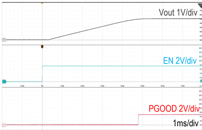
Figure 19. On/Off Enable Waveform
