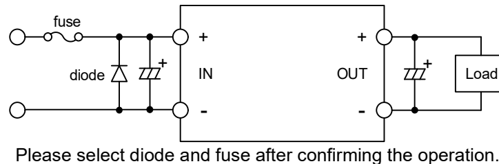
Figure 43. Circuit example with a diode and fuse
