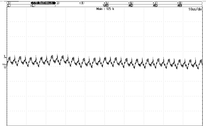
Figure 5 Ripple & Noise 48Vin, 25A Load, 470µF min cap load
