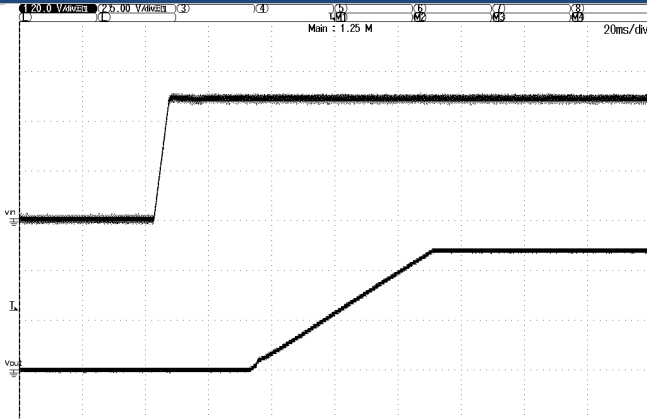
Figure 2 Vin ON 48Vin, 25A Load, 470µF min cap load
