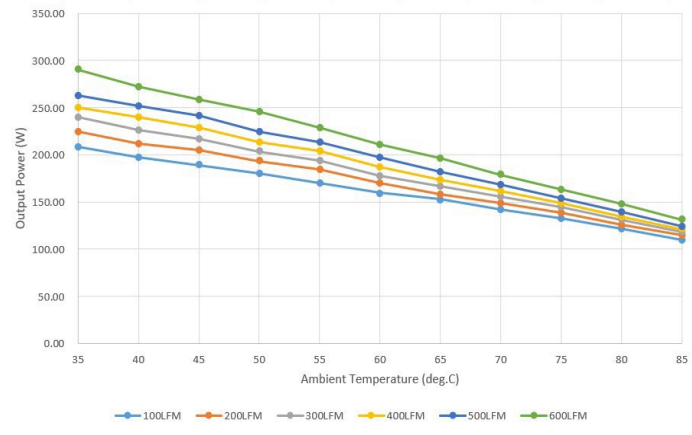
Figure 15 Temperature Derating – Longitudinal Direction Vin=48Vdc (airflow is from Vin to Vout on 10"x10" PCB, without baseplate)
