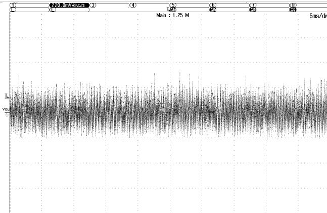
Figure 4 Ripple & Noise 48Vin, 25A Load, 470µF min cap load
