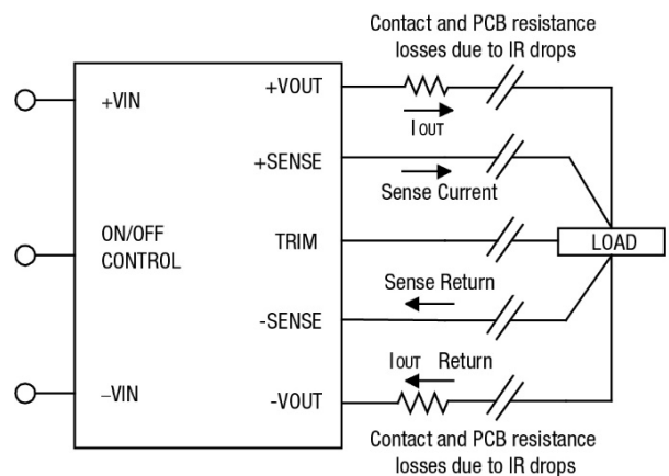
Remote Sense Circuit Configuration
