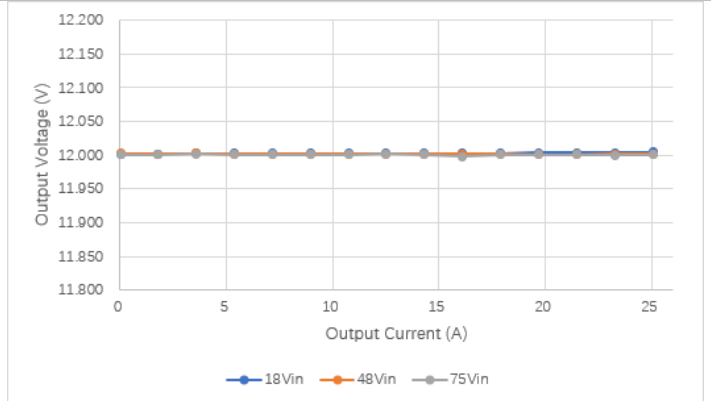
Figure 9 Output Voltage vs Output Current
