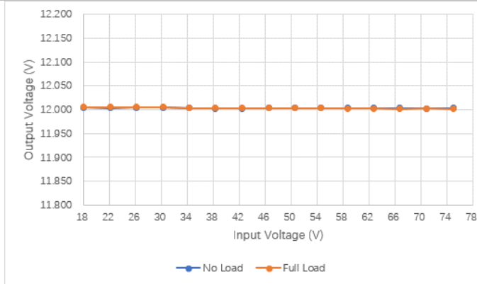
Figure 8 Output Voltage vs Input Voltage
