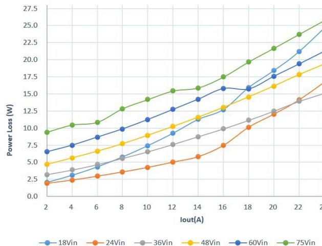
Figure 11 Power Dissipation Vs. Load Current @ 25°C
