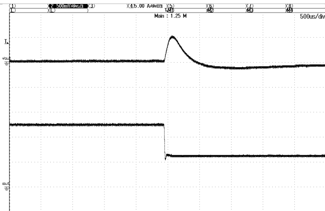
Figure 6 Output Transient Response 48Vin, 75%-50% Load, 470µF min cap load
