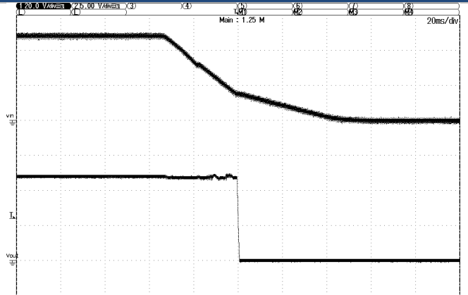
Figure 3 Vin Off 48Vin, 25A Load, 470µF min cap load
