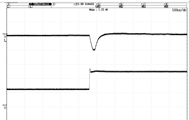
Figure 7 Output Transient Response 48Vin, 50%-75% Load, 470µF min cap load
