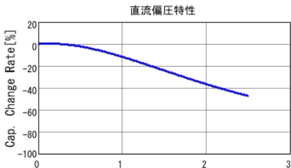
GCM155D70E106ME36 C-DC bias capchange, 25.0degC, A
