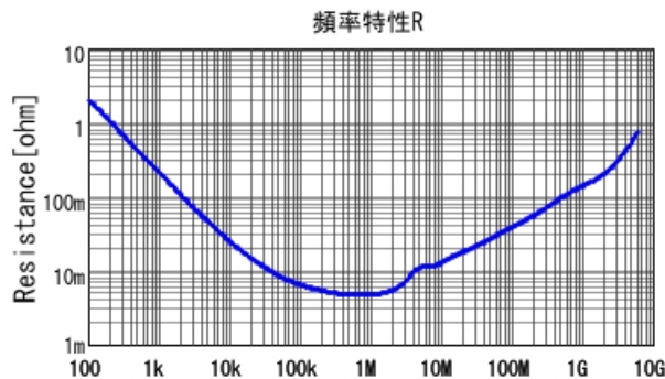
GCM155D70E106ME36 R DCOV, 25degC
