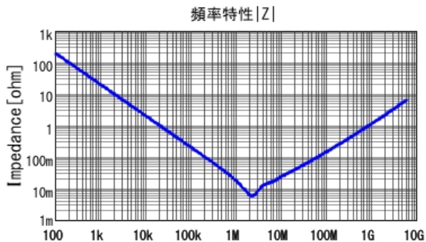
GCM155D70E106ME36 |Z| DCOV, 25degC
