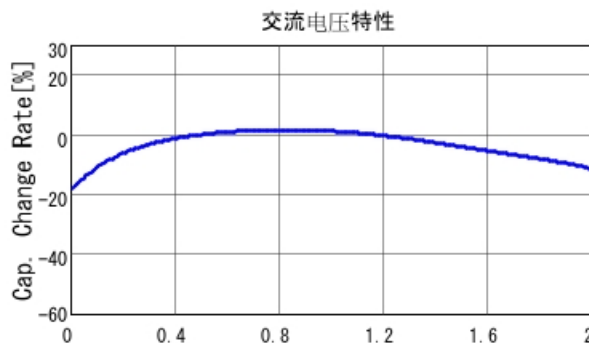
GCM155D70E106ME36 C-AC Voltage capchange, DCOV, 25
