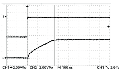
Typical Start-Up Wave Form
