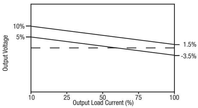
NXE1S0505MC
