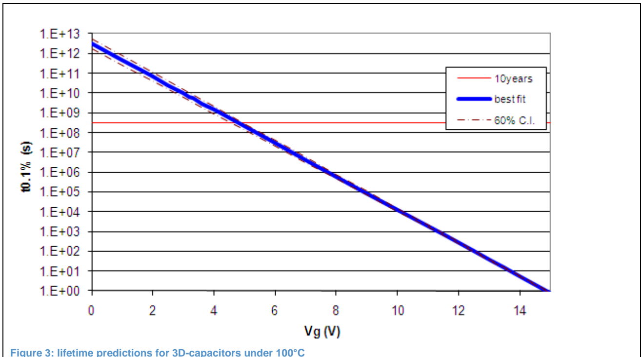
Figure 3: lifetime predictions for 3D-capacitors under 100°C
