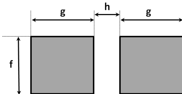
Fig. 3 Land Pattern
