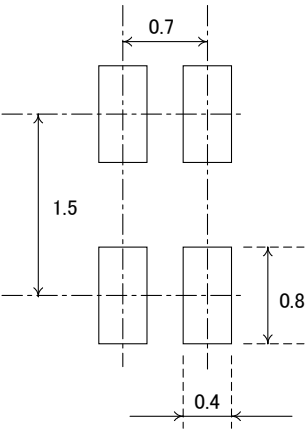
Reference mount pad
