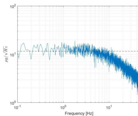
Figure 6 Example noise spectrum of Y-channel in mode 4
