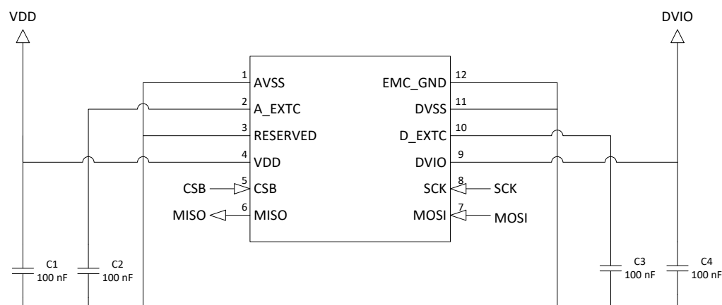
Figure 16 Application schematic.
