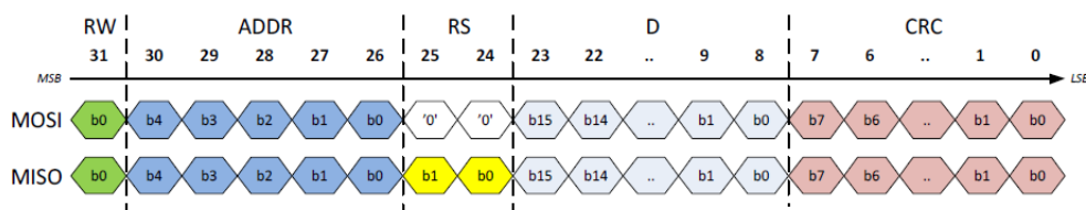
Figure 14 SPI Frame
