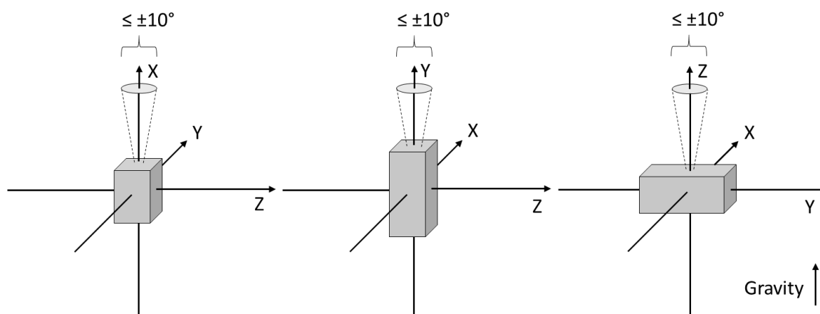
Figure 9 Measurement ranges on inclination modes (Mode 3 and Mode 4)
