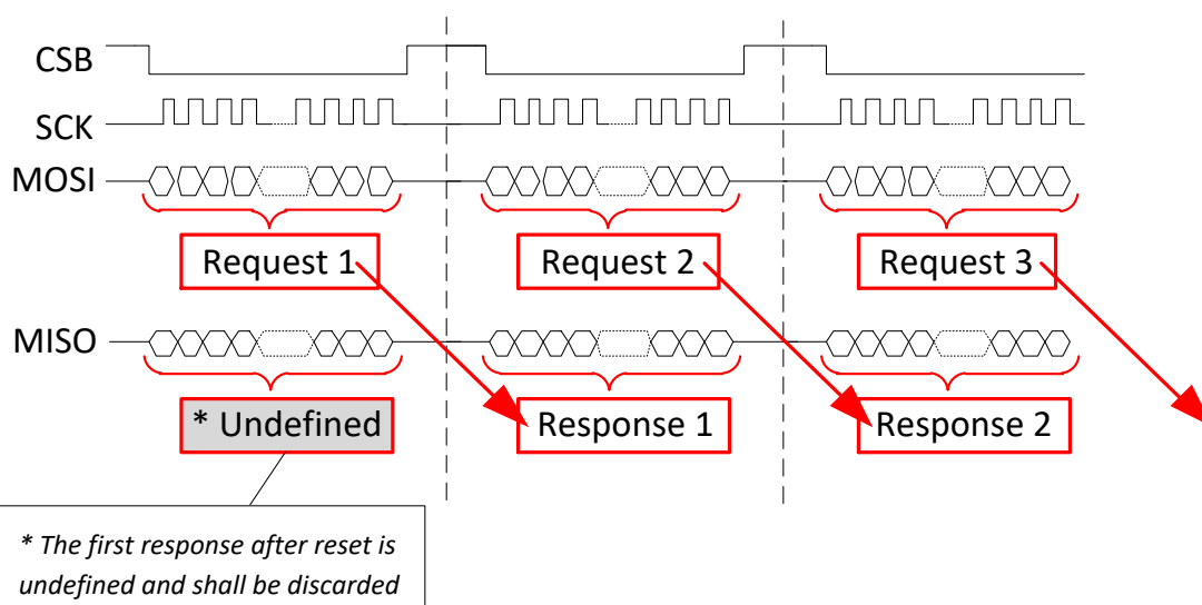
Figure 13 SPI Protocol
