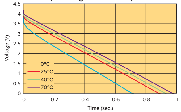
Constant Current Discharge (@25°C) (Discharge Current: 2A)
